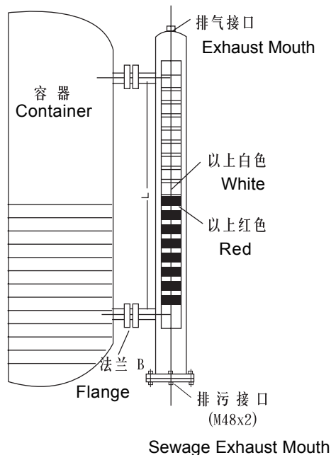
Figure 1 Working Theory
